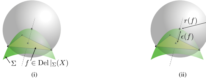
Fig. 2. The surface Delaunay ball (SDB) for a restricted 2-face f \in \text{Del}_\Sigma(X) , showing (i) placement of the surface ball at the intersection of the associated dual edge \mathbf{v}_f \in \text{Vor}(X) and the surface \Sigma , and (ii) associated SDB radius r(f) and surface discretisation error \epsilon(f) .
